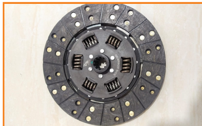
ECOMATE CLUTCH DISC
